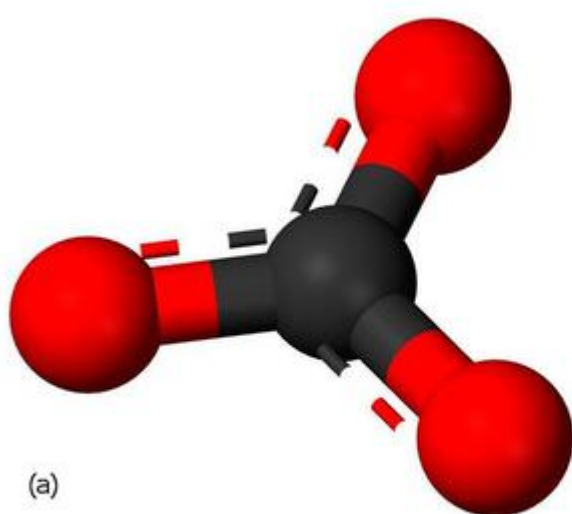
(a) The carbonate ion is one carbon atom bonded to three oxygen atoms.
