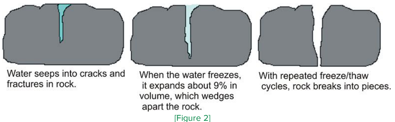
Ice wedging.
